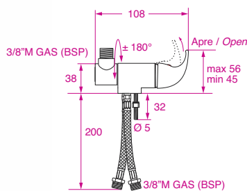
Maniglia / Handle KNB-ML2XX
