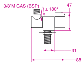
Maniglia / Handle KNB-RR/MR
