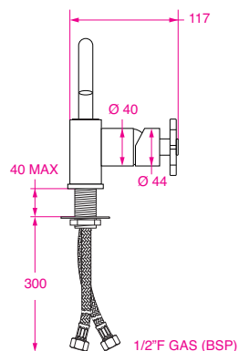
VISTA FRONTALE / FRONT VIEW
